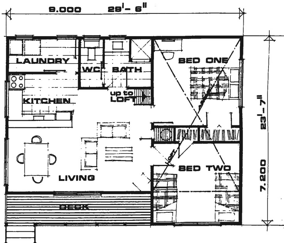
PLAN NO. 1 844 APPROX SQ. FT. 3 BEDROOMS DECK INCLUDED
